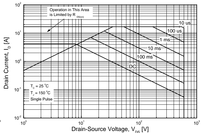
TMPF5N60Z(G)
