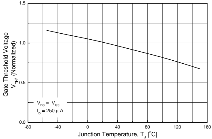
TMPF5N60Z(G)
